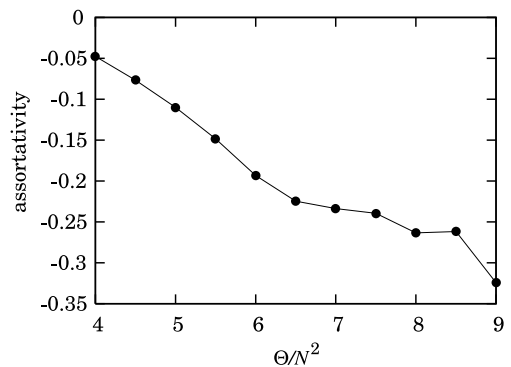
図4 結合相関 Fig.4 Degree correlation.
