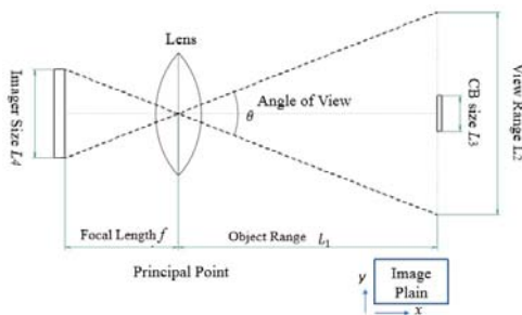
Figure 14: Pinhole Camera Model
