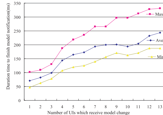
Fig. 15 Notification time of changed-model to all UIs.
