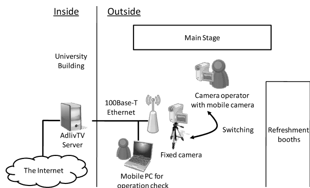
Fig. 9 Network configuration in the campus festival.
