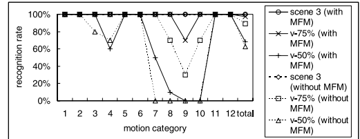
Fig. 17 Comparison of recognition rates for vertical scaling-down.
