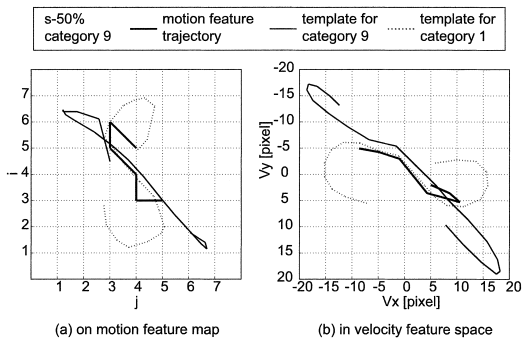
Fig. 29 Example of the recognition failure due to small velocity.
