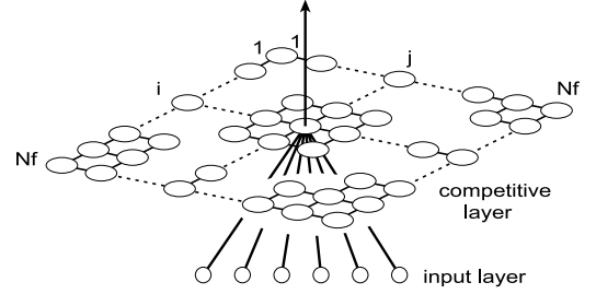
Fig. 4 Structure of the 2-D topological SOM.
