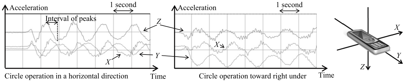
Fig. 4 Examples of the acceleration of the circle operation.
