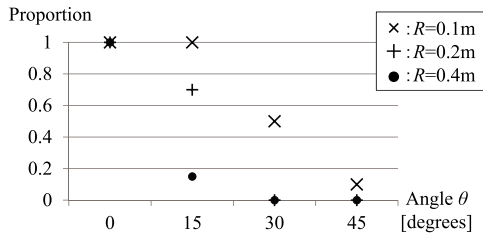
Fig. 13 Results in the case of the radius R of 0.1, 0.2, and 0.4 meters.
