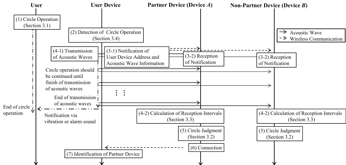
Fig. 5 Entire procedure of the user and the neighborhood devices.
