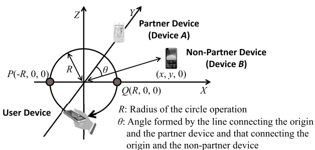
Fig. 6 Supposed condition for analysis of the resolution.
