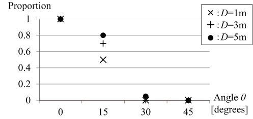
Fig. 11 Results when distance D between devices is 1, 3, and 5 meters.
