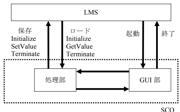
(b) SCORM 2004
