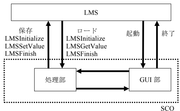
(a) SCORM 1.2
