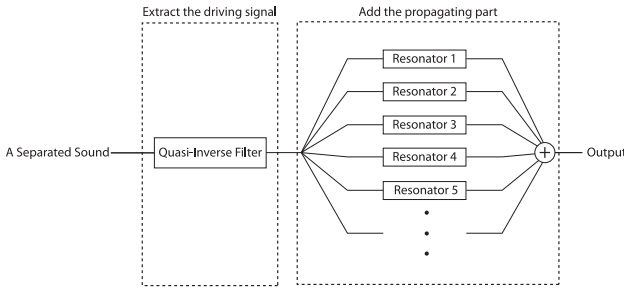
Fig. 7 Quasi-inverse filter block and synthesis block.
