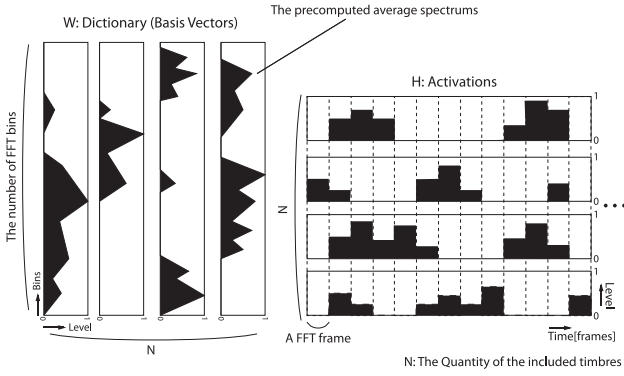
Fig. 6 Dictionary matrix and activation matrix.
