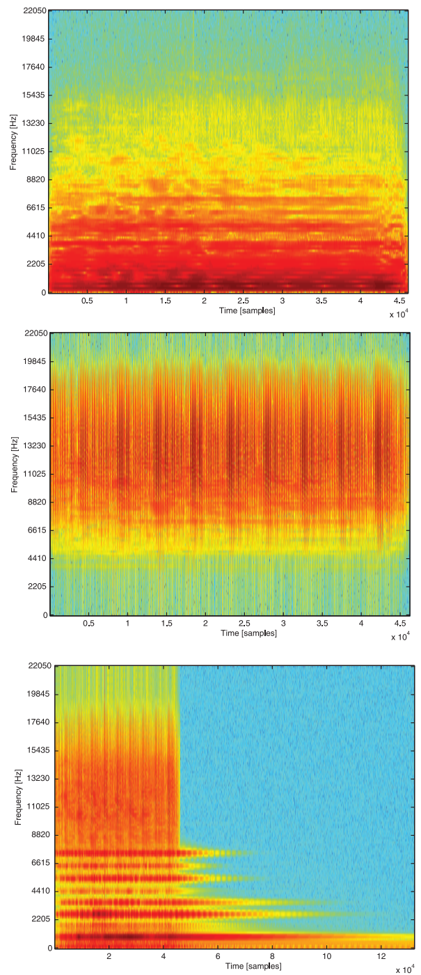
Fig. 10 Assigning a piano A4 timbre to a violin long tone with vibrato. Top: The violin E6 long tone with vibrato (the target) Middle: The extracted driving signal from the target. Bottom: The synthesized result.
