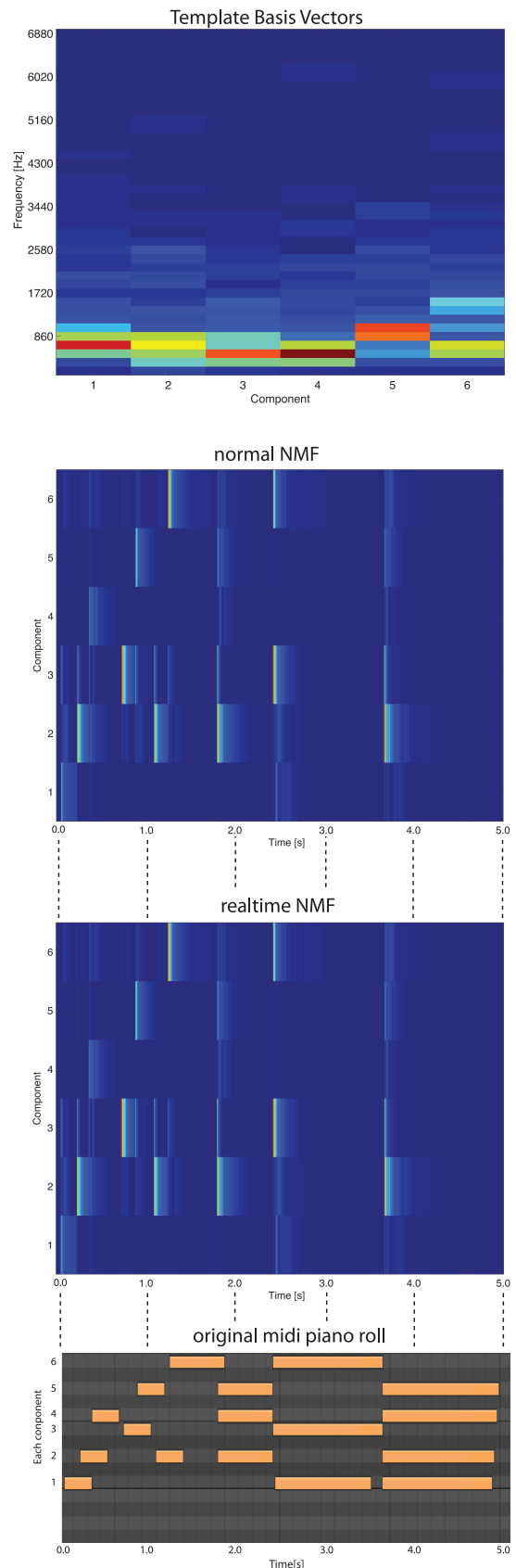
Fig. 8 The result of the sound source separation test. Top: The dictionary matrix used for template Second: The activation matrix of Normal NMF Third: The activation matrix of Real-time NMF Bottom: The MIDI piano roll of the input source. The orange bar indicates that the corresponding timbre is sounding.
