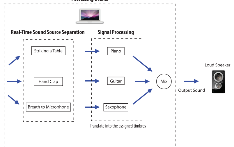
Fig. 3 The outline of possessing drums. First, the sound from the microphone is separated into each target. Second, each separated sound is modified by signal processing to translate the timbre into the assigned timbre.
