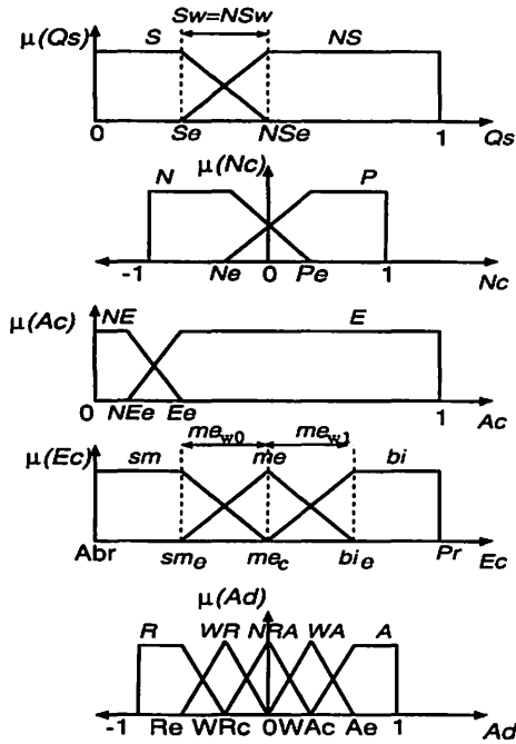
Figure 3: FAC membership functions.
