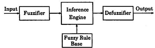
Figure 1: FLC structure.
