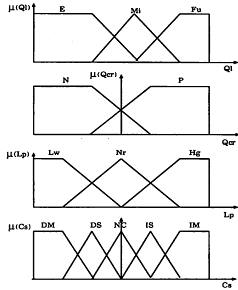
Figure 8: FCC membership functions.
