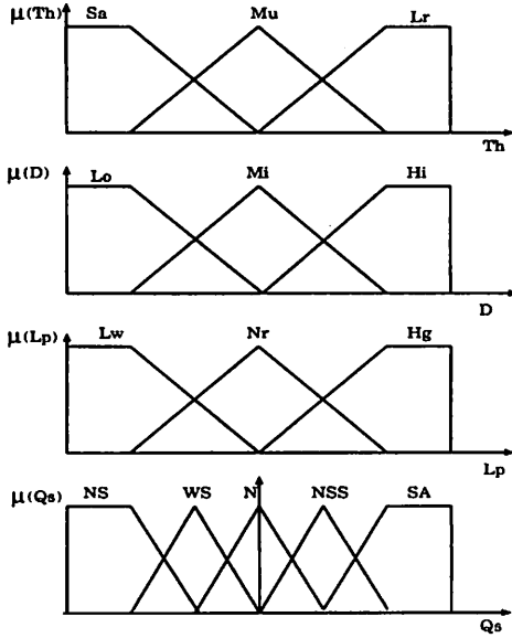
Figure 7: FQC membership functions.
