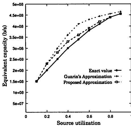
Figure 9: Performance comparison between Guérin's method and FECE.
