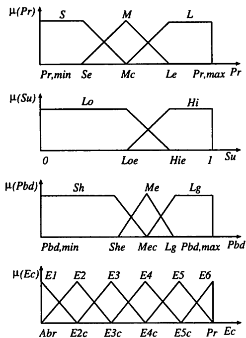
Figure 5: FECE membership functions.
