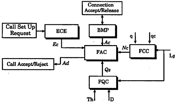
Figure 6: Proposed MFAC scheme.
