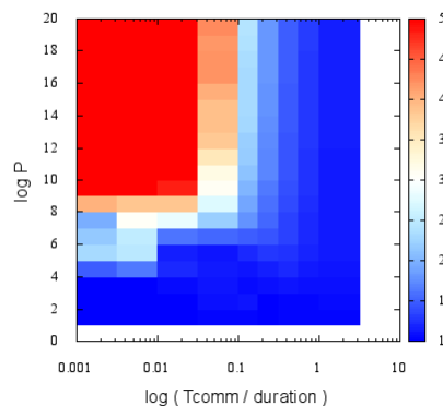
図 9 ジッタの影響 (Z 軸の範囲 [1,5]) (ジッタありの従来手法の計算時間) / (ジッタなしの従来手法の計算時間) (period=1.0e-2, duration=1.0e-4) Fig. 9 the influence of the jitter (z range [1,5]) (the computation time of the butterfly algorithm with jitter) / (the computation time of the butterfly algorithm with jitter) (period=1.0e-2, duration=1.0e-4)
