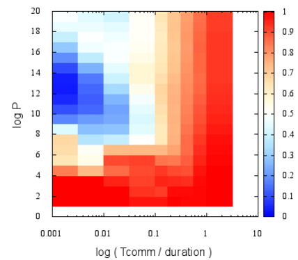
図 10 従来手法と比較した提案手法の効果 (提案手法の計算時間) / (従来手法の計算時間) (period=1.0e-2, duration=1.0e-4) Fig. 10 the effectiveness of the proposed algorithm compared to the butterfly algorithm. (the computation time of the proposed algorithm) / (the computation time of the proposed algorithm) (period=1.0e-2, duration=1.0e-4)
