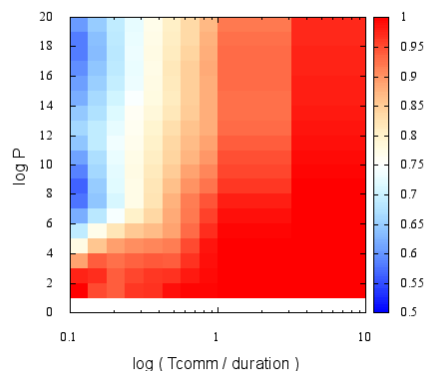
図 6 従来手法と比較した提案手法の効果 (提案手法の計算時間) / (従来手法の計算時間) (period=1.0e-3, duration=1.0e-5) Fig. 6 the effectiveness of the proposed algorithm compared to the butterfly algorithm. (the computation time of the proposed algorithm) / (the computation time of the proposed algorithm) (period=1.0e-3, duration=1.0e-5)
