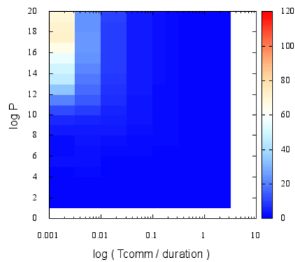
図 8 ジッタの影響 (Z 軸の範囲 [0,120]) (ジッタありの従来手法の計算時間) / (ジッタなしの従来手法の計算時間) (period=1.0e-2, duration=1.0e-4) Fig. 8 the influence of the jitter (the z range [0,120]) (the computation time of the butterfly algorithm with jitter) / (the computation time of the butterfly algorithm with jitter) (period=1.0e-2, duration=1.0e-4)
