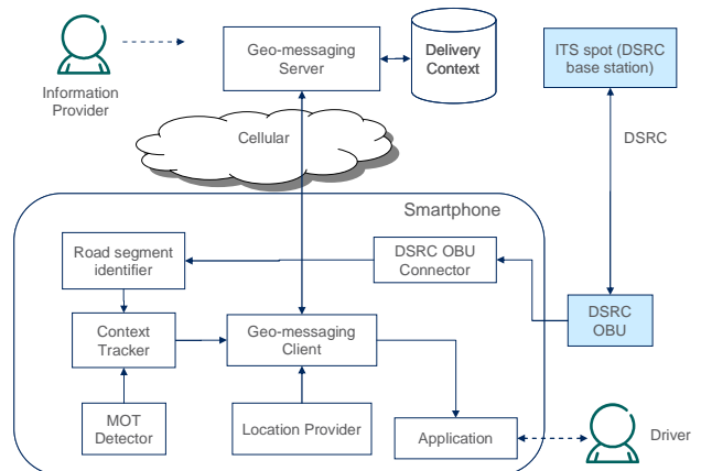
Fig. 3 Solution architecture alternative 2.
