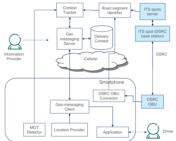
Fig. 2 Solution architecture alternative 1.
