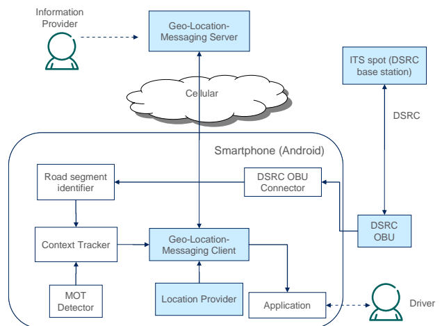
Fig. 7 Prototype of the 2 nd architecture alternative.
