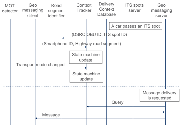
Fig. 4 Sequence diagram of alternative 1.
