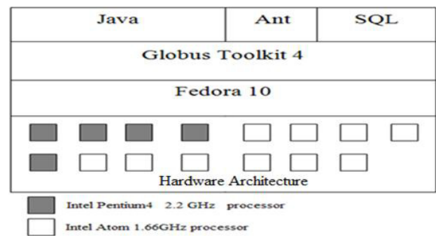
Fig. 6 Experimental platform.
