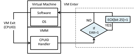
Figure 2: How to fake CPUID
