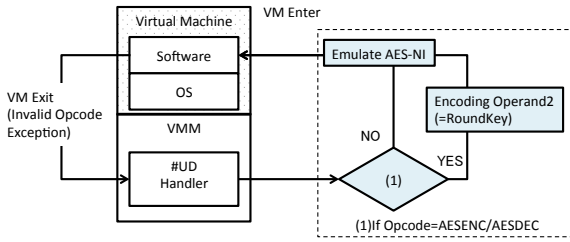
Figure 3: Exception Handling on VMM
