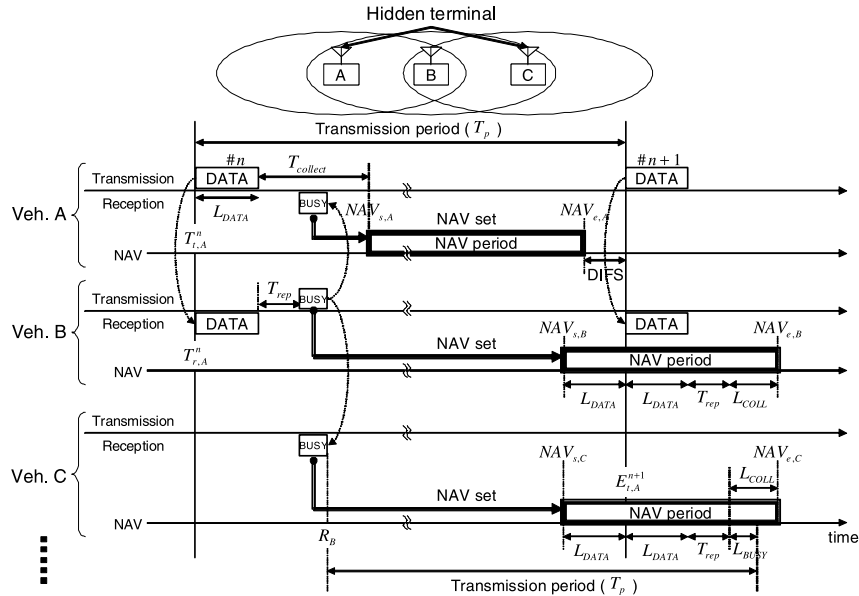
Fig. 4 Hidden terminal detection and packet collision avoidance method.
