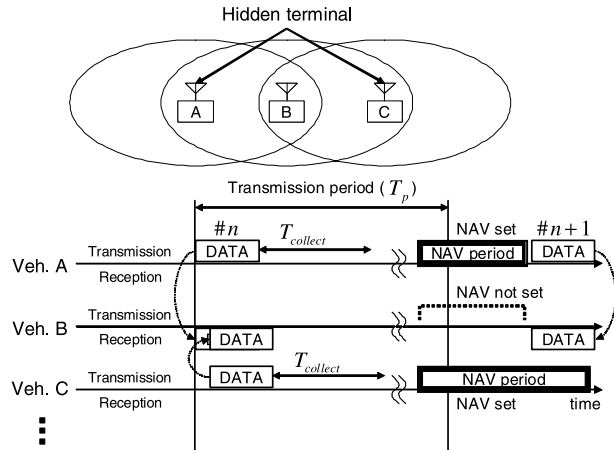
Fig. 11 Algorithm of the PB-TRMA only BUSY scheme for the case in which DATA packet collisions occur.
