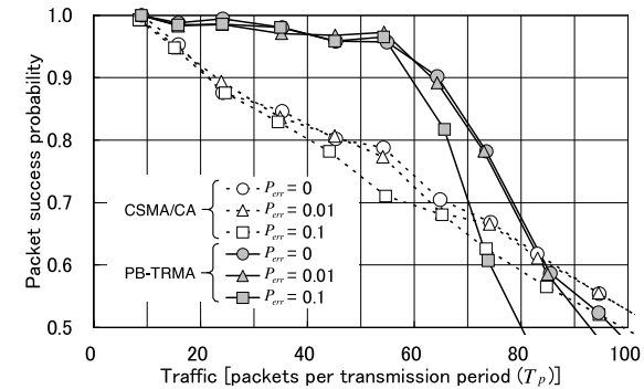
Fig. 15 Effect of packet error on PB-TRMA and CSMA/CA.
