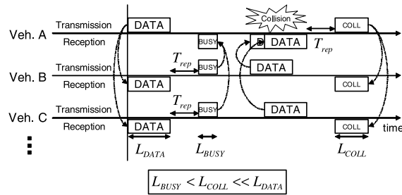
Fig. 2 Basic concept of PB-TRMA.
