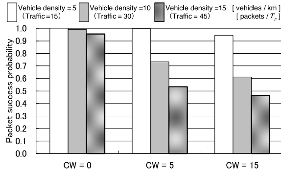
Fig. 8 Packet success probability for CW in PB-TRMA.
