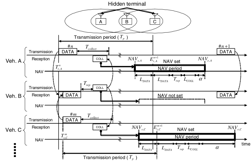
Fig. 3 Packet collision retrieval method in PB-TRMA.
