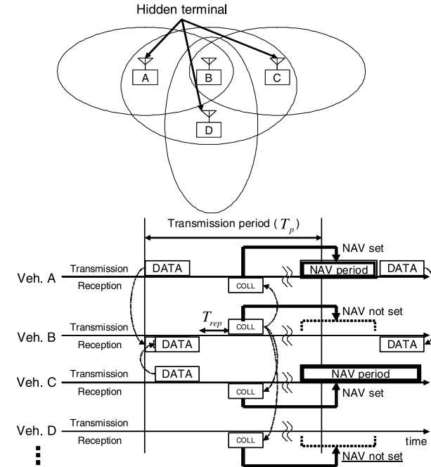
Fig. 5 Hidden terminal detection by receiving COLL.
