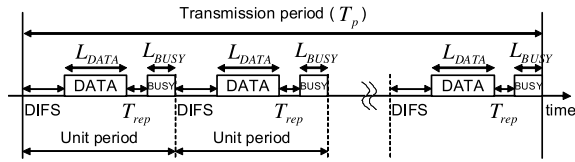
Fig. 16 Maximum number of DATA during one transmission period for PB-TRMA.
