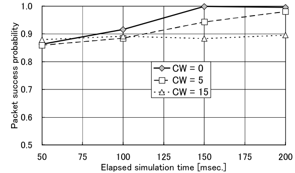
Fig. 9 Packet success probability for elapsed simulation time.
