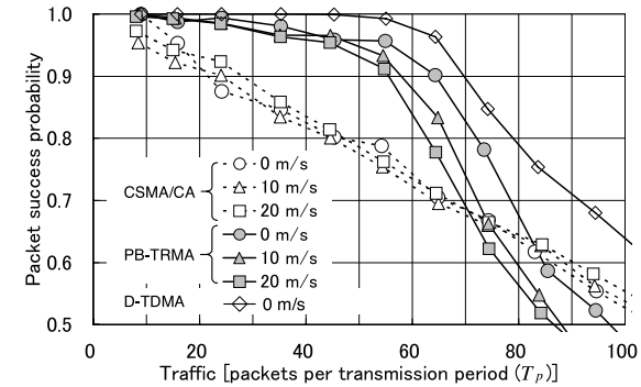
Fig. 17 Performances of PB-TRMA, D-TDMA and CSMA/CA.
