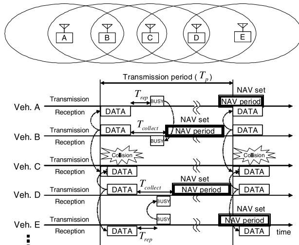
Fig. 14 Successive packet collisions in the PB-TRMA only BUSY scheme.
