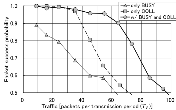
Fig. 13 Packet success probability for communication traffic in PB-TRMA.
