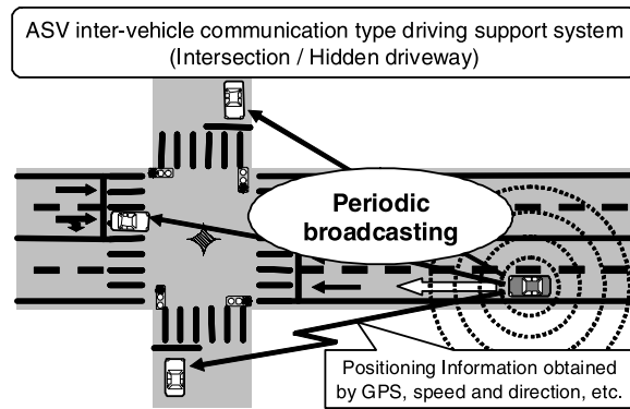
Fig. 1 Inter-vehicle communication system for safety.
