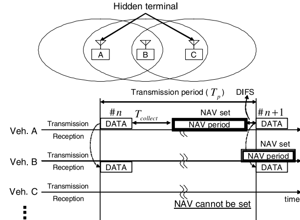
Fig. 12 Algorithm of the PB-TRMA only COLL scheme for the case in which the DATA packet is received correctly.
