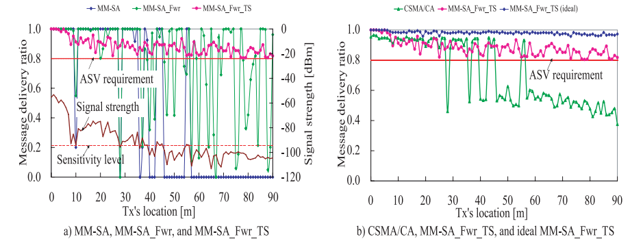
Fig. 9 Comparing delivery performances for encounter collision scenario (176 vehicles).
