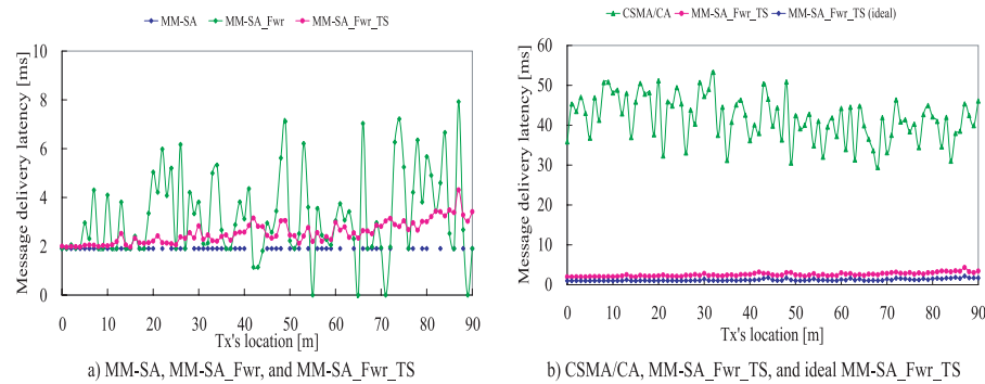
Fig. 17 Comparing delay performances for right-turning collision scenario.
