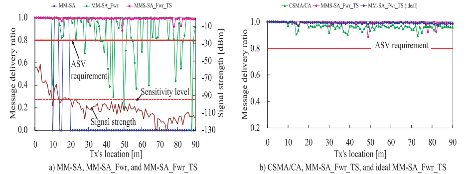
Fig. 8 Comparing delivery performances for encounter collision scenario (88 vehicles).
