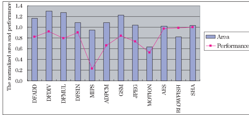
Fig. 4 Sensitivity of area and execution cycles to resource constraint.
