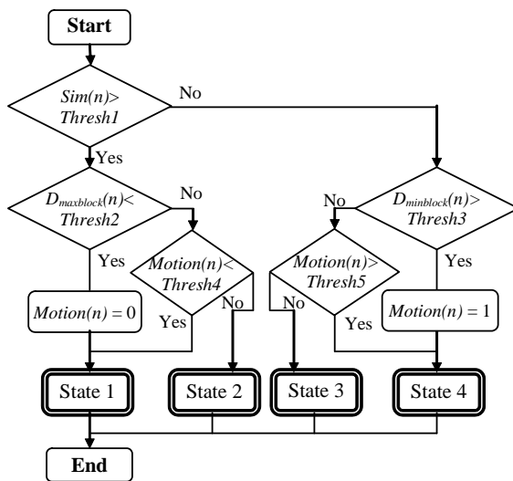
Fig. 7 A decision tree for classifying states.
