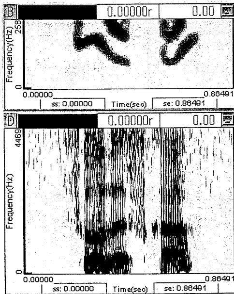
Figure 2. Spectrograms of /soHdesuka/ uttered with the paralinguistic meaning of "(D) indifference". 527ms long.
