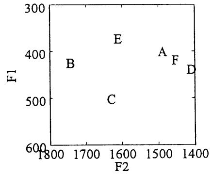
Figure 9. F1-F2 scatter plot of the six realizations of /e/.
