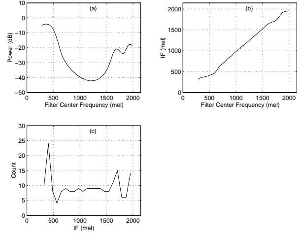
Fig. 2: (a) Short-time power spectrum P(\nu_i, t) , (b) Short-time IF spectrum F(\nu_i, t) , and (c) Short-time IF histogram H(F, t) .
