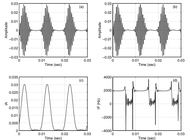
图 1: (a) Filtered signal s(\nu_i, t) from the i -th bandpass filter with center frequency \nu_i = 1880 Hz and bandwidth = 280 Hz, (b) Hilbert transform \hat{s}(\nu_i, t) , (c) IA function a(\nu_i, t) , and (d) IF function f(\nu_i, t) .
