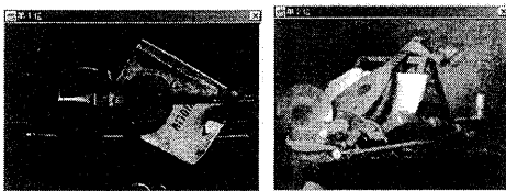
(b) H = 0.60002
