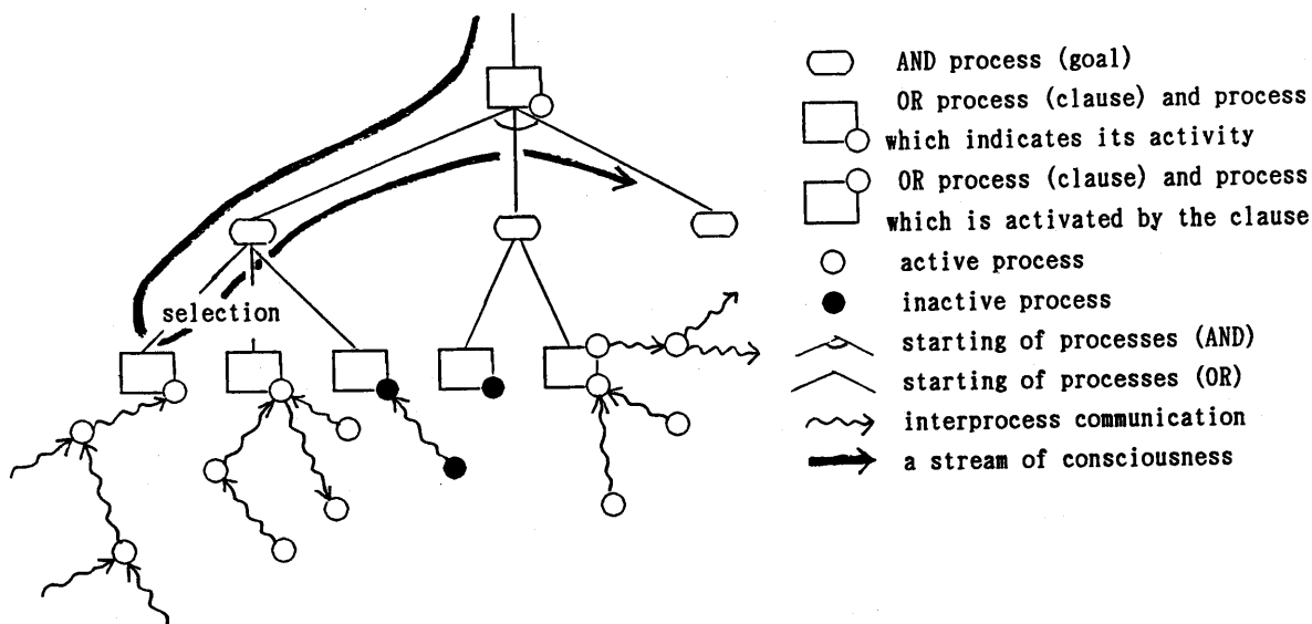
Figure 2: The computation in the C/U model
