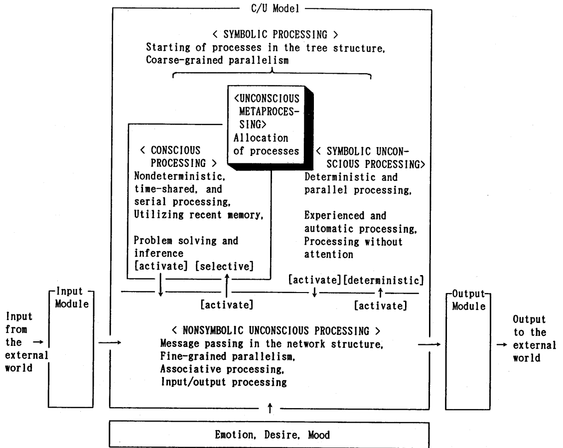
Figure 1: The structure of the C/U model
