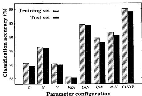
Figure 2: Evaluation of different parameter settings
