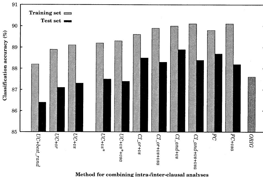
Figure 1: Evaluation of the different clause processing configurations
