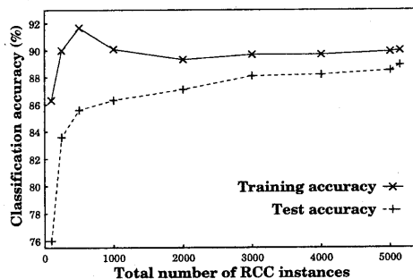
Figure 3: Learning curve
