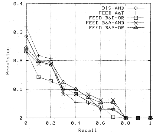
Figure 5. Recall-Precision Curves for QE experiments via Feedback loops
