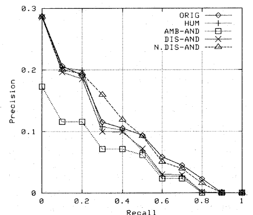
Figure 4. Recall-Precision Curves for QT/D experiments
