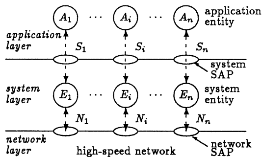
図1: 群 C = \langle E_1, \dots, E_n \rangle
