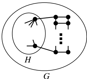
Fig. 5 A case that 2-edge-connected induced subgraph H of an input graph G has exponential child-candidates.
