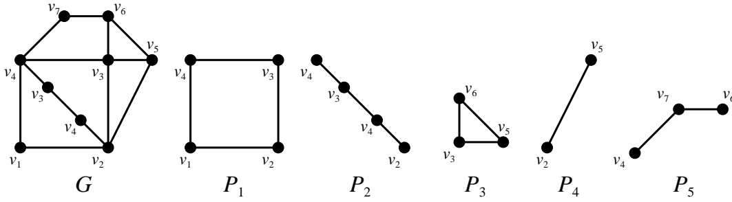
Fig. 1 An example of a closed-ear decomposition. The graph G has a closed-ear decomposition P_1, P_2, P_3, P_4, P_5 .
