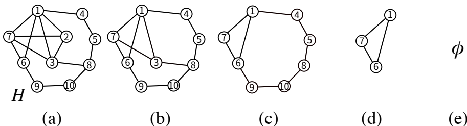
Fig. 3 An example of the parent sequence of a 2-edge-connected induced subgraph. (a) A 2-edge-connected induced subgraph H . (b) The parent \mathcal{P}(H) of H . \mathcal{P}(H) is obtained from H by removing \{2\} . (c) The parent \mathcal{P}(\mathcal{P}(H)) of \mathcal{P}(H) . \mathcal{P}(\mathcal{P}(H)) is obtained by removing \{3\} . (d) The parent \mathcal{P}(\mathcal{P}(\mathcal{P}(H))) of \mathcal{P}(\mathcal{P}(H)) . \mathcal{P}(\mathcal{P}(\mathcal{P}(H))) is obtained by removing \{4, 5, 8, 10, 9\} . (e) Finally, the root, the empty graph, is obtained by removing \{1, 6, 7\} .
