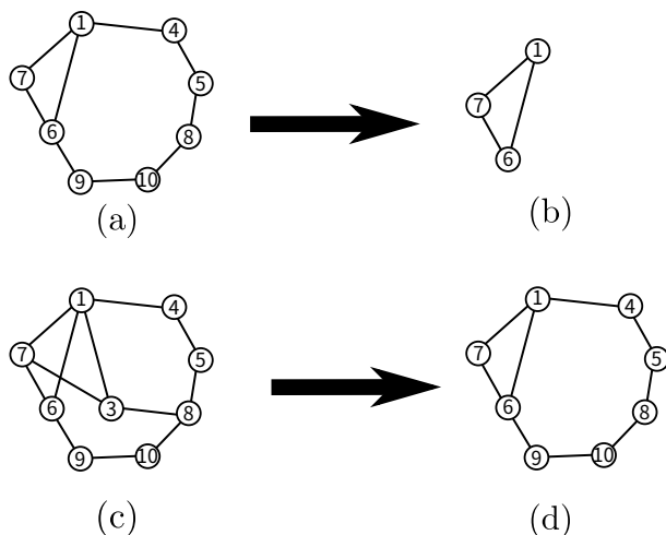
Fig. 2 (a) A 2-edge-connected induced subgraph H_1 . (b) The parent \mathcal{P}(H_1) of H_1 . \mathcal{P}(H_1) is obtained from H_1 by removing \{4, 5, 8, 10, 9\} , which is the smallest minimal removable set of H_1 . (c) A 2-edge-connected induced subgraph H_2 . (d) The parent \mathcal{P}(H_2) of H_2 . \mathcal{P}(H_2) is obtained from H_2 by removing \{3\} , which is the smallest minimal removable set of H_2 .
