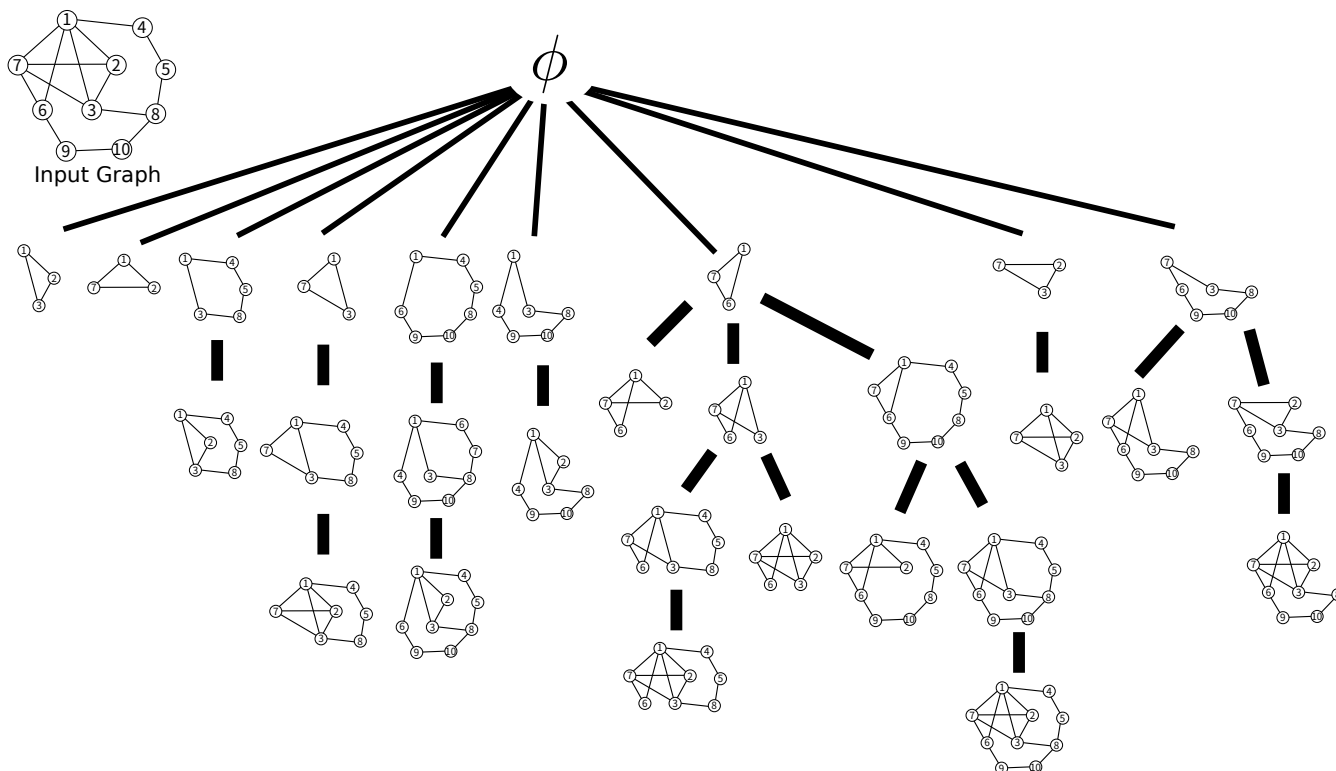
Fig. 4 An example of family tree of the input graph, drawn in the upper-left of the figure.
