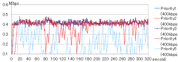
(b) Receive rate of UDP flows
