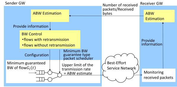
Fig. 3 Structure of GWs that eR2BC assumes.
