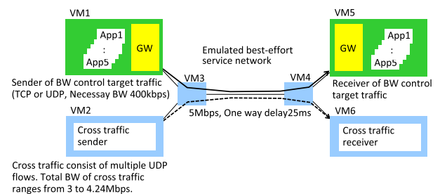
Fig. 10 Structure of virtual machines for evaluation.
