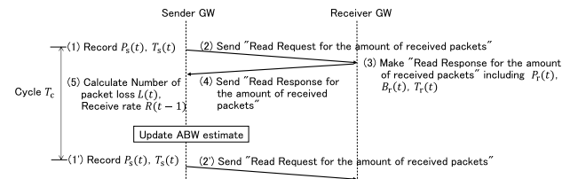
Fig. 9 Procedure to obtain information necessary for packet loss detection.
