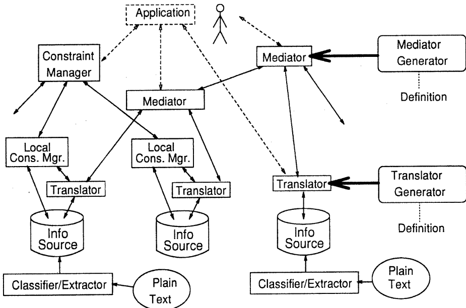
Figure 1: Tsimmis Architecture
