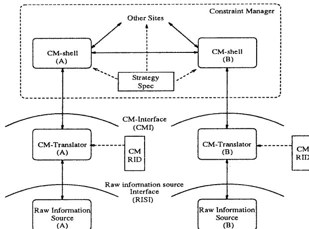
Figure 6: Constraint Management Toolkit Architecture
