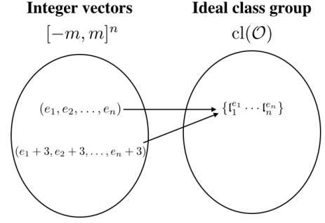
Fig. 2 Collision in the ideal representation
