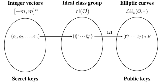
Fig. 1 Correspondence of keys in CSIDH
