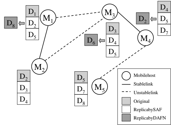
Figure 2: Result of the SAF and DAFN-S1 or DAFN-S2 methods.
