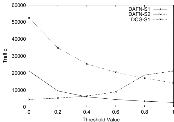
Figure 12: Threshold value and traffic (Case 1).
