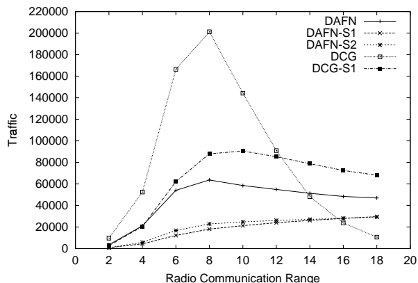
Figure 9: Radio communication range and traffic (Case 1).
