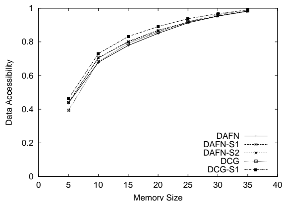
Figure 7: Memory size and data accessibility (Case 1).
