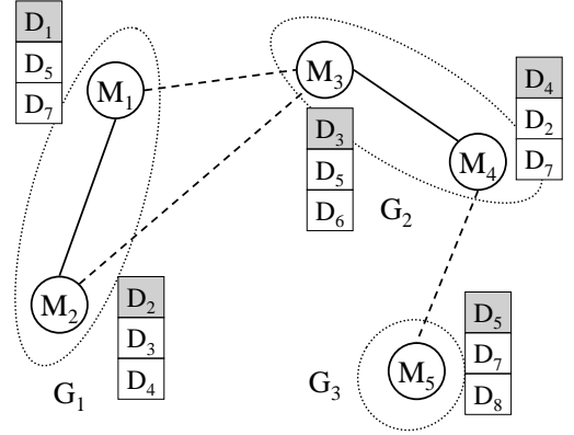
Figure 3: Result of the DCG-S1 method.
