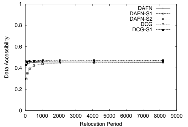
Figure 5: Relocation period and data accessibility (Case 1).
