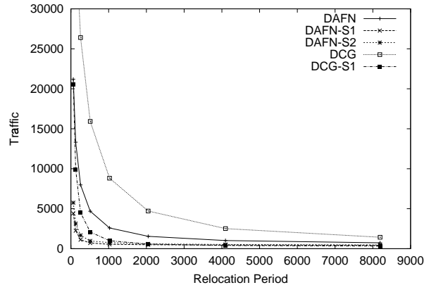
Figure 6: Relocation period and traffic (Case 1).
