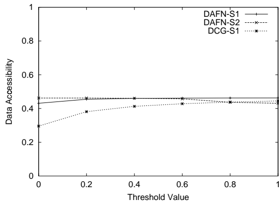
Figure 11: Threshold value and data accessibility (Case 1).
