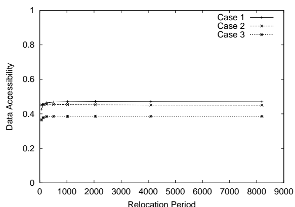
Figure 10: Relocation period and data accessibility for three different cases of data access patterns in the DCG-S1 method.
