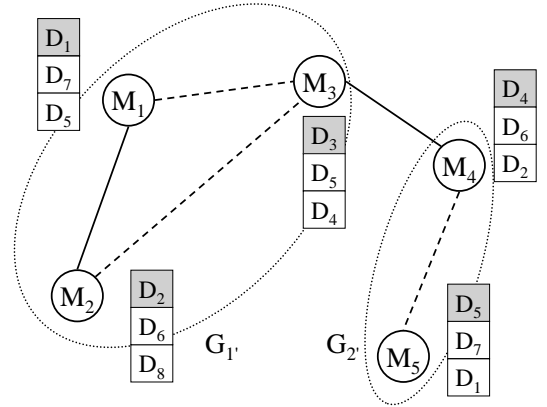
Figure 4: Result of the DCG method.
