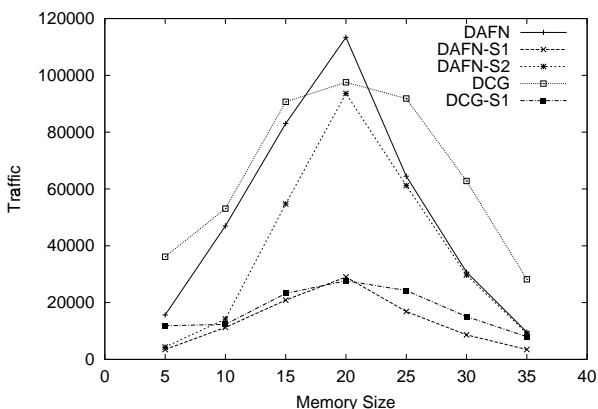
Figure 8: Memory size and traffic (Case 1).
