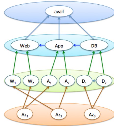
Fig. 1. A Bayesian network to model of availability
