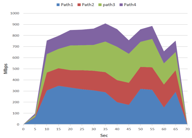
Fig. 11 Used bandwidth for the round robin assignment method in case of using 24 parallel TCP streams (6 parallel TCP streams are assigned for each path).
