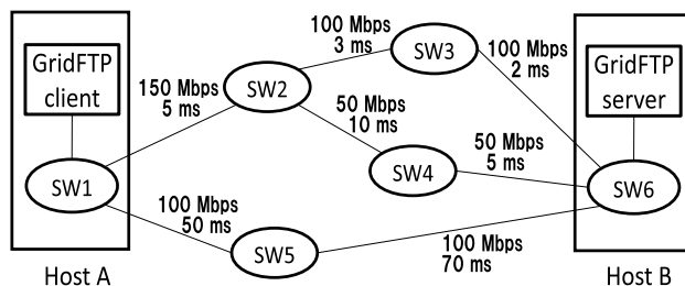
Fig. 4 Topology B on a local testbed (different bandwidth and latency are configured for each path as shown in the Figure).
