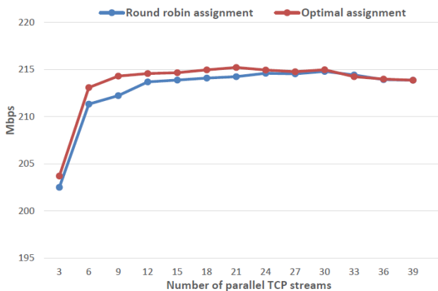
Fig. 8 Comparison of the average data transfer speed between the optimal assignment and the round robin assignment in topology B.
