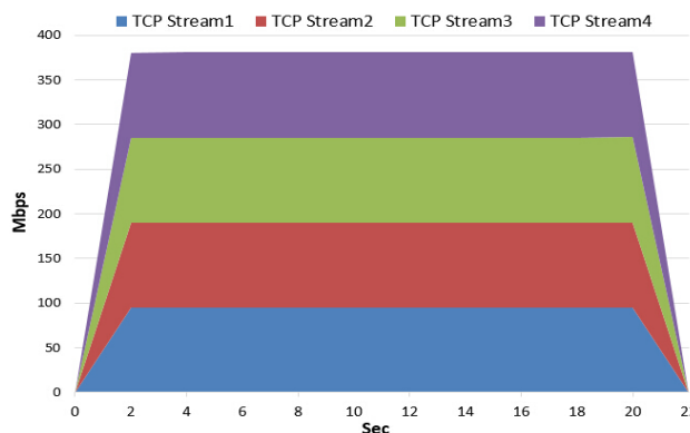
Fig. 7 Used bandwidth of each TCP stream in topology A with four parallel TCP streams.
