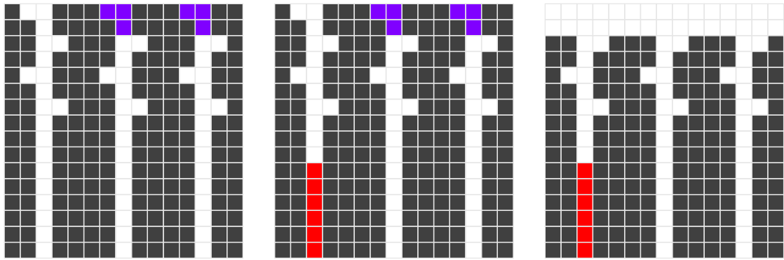
Fig. 4 Placing a_i = 2 in Fig. 3.
