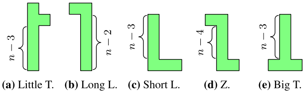
Fig. 17 The pieces used in the n -tris hardness proof for n > 5 . Note the number of rows in each piece is at least 4 for all n \geq 6 , so each piece has at most two possible orientations to fit in a bucket. The Z piece (d) is the same after being rotated 180^\circ , so it has only one possible orientation.
