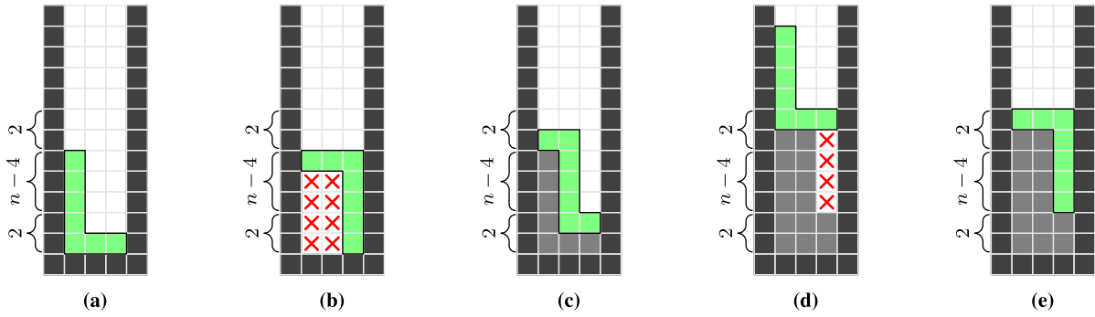
Fig. 22 The filler sequence. Figures 22 (a) and 22 (b) show the two possible orientations for the first filler piece, only one of which is valid. Figure 22 (c) shows how the only possible orientation for the second filler piece fits on top of the only valid position for the first filler piece. Figures 22 (d) and 22 (e) show the two possible orientations for the third and final filler piece, only one of which is valid.
