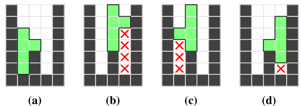
Fig. 11 Possible positions for the little T piece (the first priming piece) in an unprimed bucket. Clearly, only one placement is valid.
