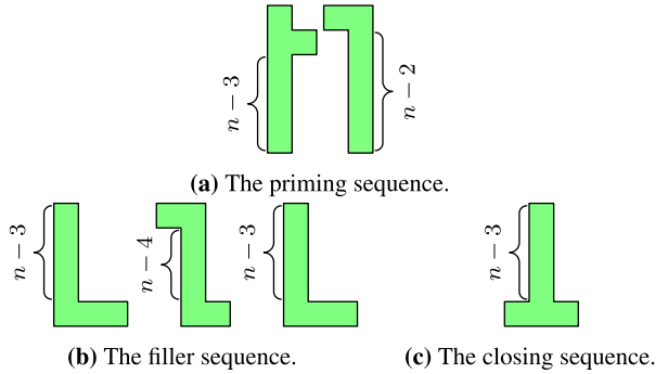
Fig. 18 The sequences of pieces used for the n -tris proof.
