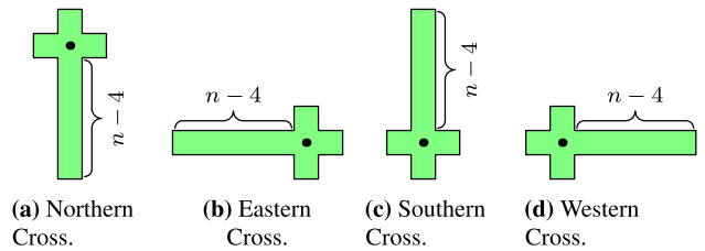
Fig. 25 The piece used to construct an unwinnable sequence for n -tris, n > 5 . The "center" of each is drawn with a dot. Note that this may or may not be the center of rotation of the piece — for this proof, rotation does not matter.
