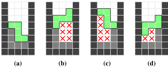
Fig. 14 Possible positions for the Z piece (the second piece in the filler sequence), given the two valid positions for the first piece in the filler sequence.
