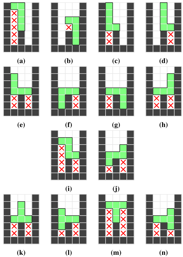
Fig. 10 Figures (a) through (d) show what happens if the long L piece (the second priming piece) is placed in an unprimed bucket. Figures (e) through (h) show what happens if the short L piece (the first and last filler piece) is used in an unprimed bucket. Figures (i) through (j) show what happens if the Z piece (the second filler piece) is used in an unprimed bucket. Figures (k) through (n) show what happens if the big T piece (the closing piece) is used in an unprimed bucket. Note that all possible configurations will result in holes or choke points, meaning the player will not be able to win.
