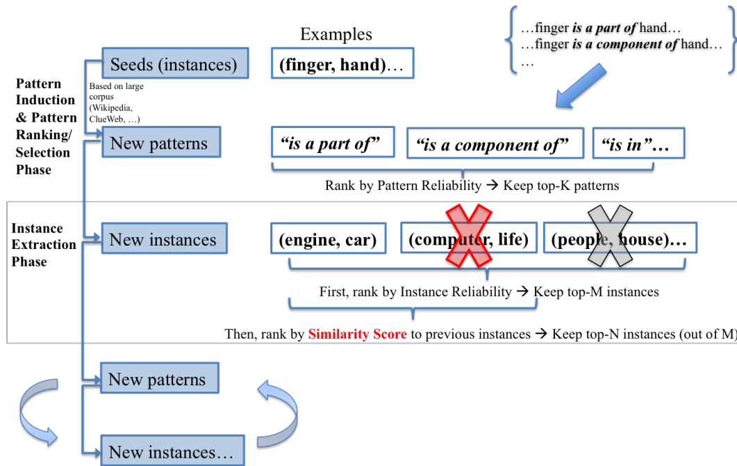
Fig. 1 Illustration of our proposed model (Espresso + Word2vec)
