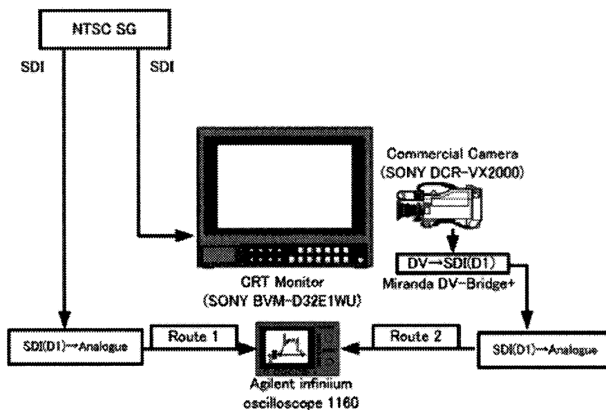
Figure 1: System to Measure the Signal Characteristics
