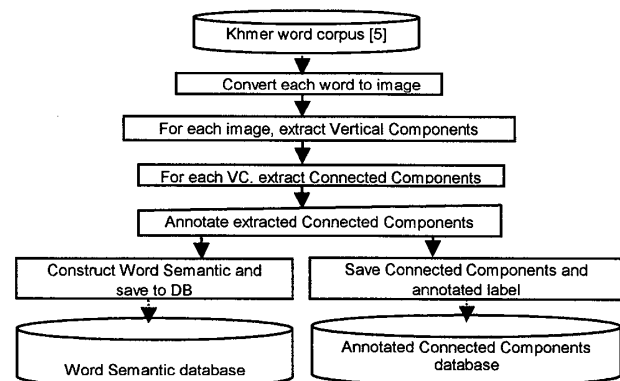
Fig.1. Word Semantic annotation flowchart
