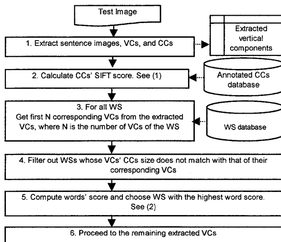
Fig.5 Recognition flowchart
