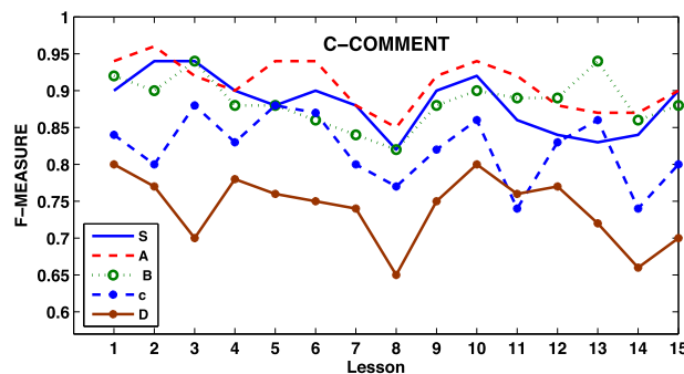
(b) Prediction results for C-comment
