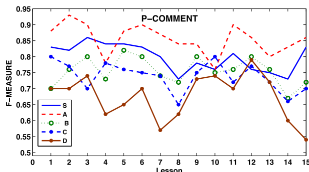
(a) Prediction results for P-comment
