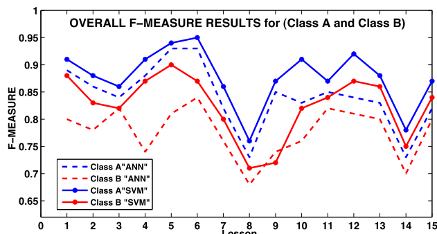
Fig. 8 Overall F -measure results for C-comments in class A and class B.
