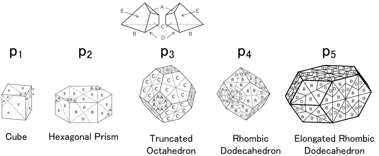
Fig. 4 Parallelohedra as pentadral complexes.
