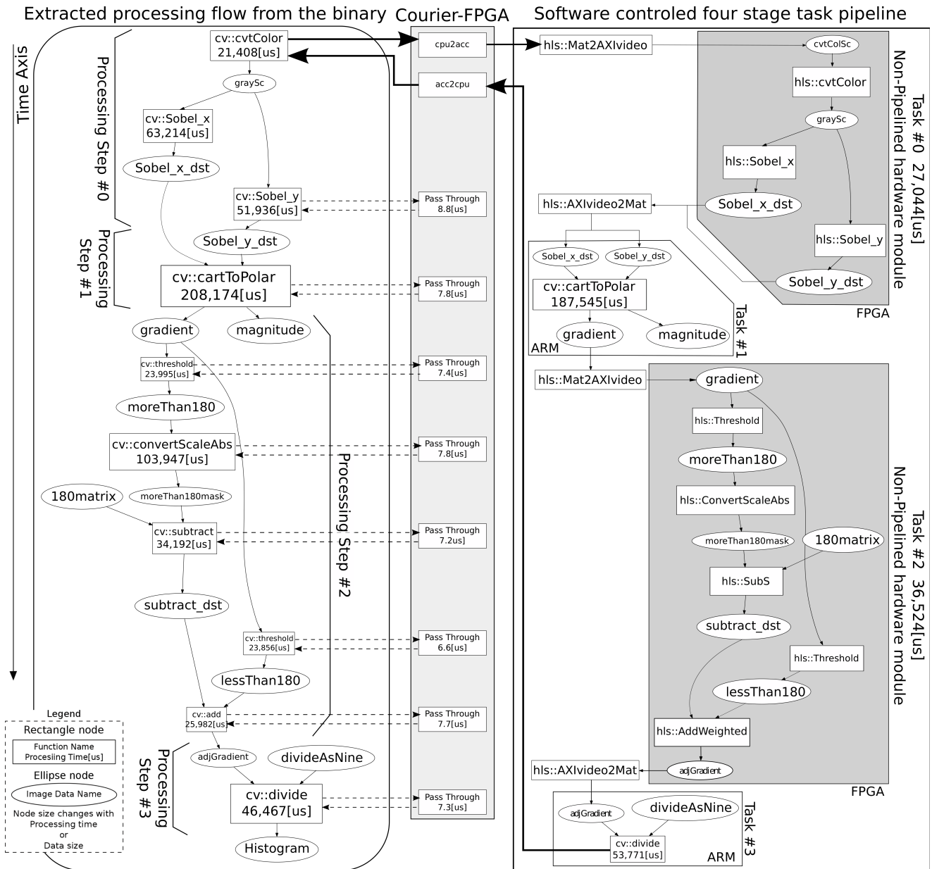
Fig. 4 Processing flow extracted from the running binary (left) and off-loaded flow (right). Each processing step is assigned to a task. The Function Off-loader generates a four stage mixed software hardware pipeline.
