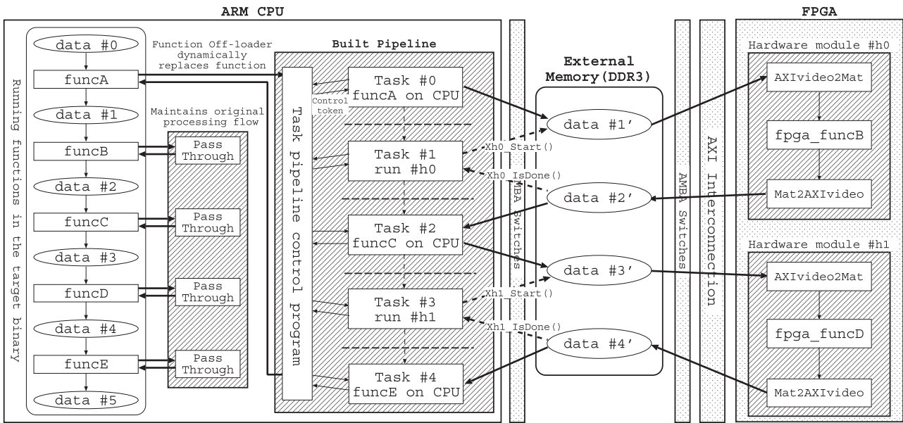
Fig. 3 Behavior of a typical mixed software hardware pipeline controlled by software program. Shaded rectangles are generated by Pipeline Generator. Tasks run in a pipelined manner, and each task can send and receive input and output data which is indicated by bold line. Input and output data of tasks are stored in the external memory. In this case, Task #1 and #3 run hardware module #h0 and #h1 while Task #0, #2 and #4 run software function.
