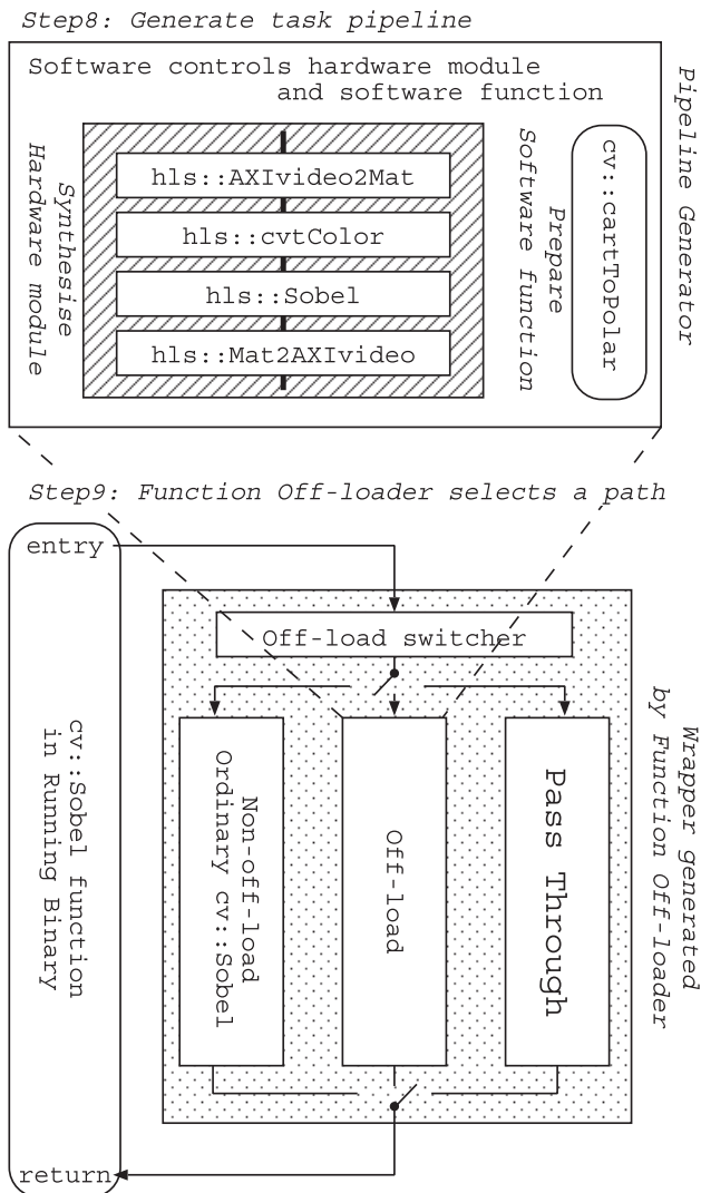
Fig. 2 In step 8, the Pipeline Generator prepares a mixed software hardware task pipeline. In step 9, the Function Off-loader uses the pipeline when “off-load” is selected.
