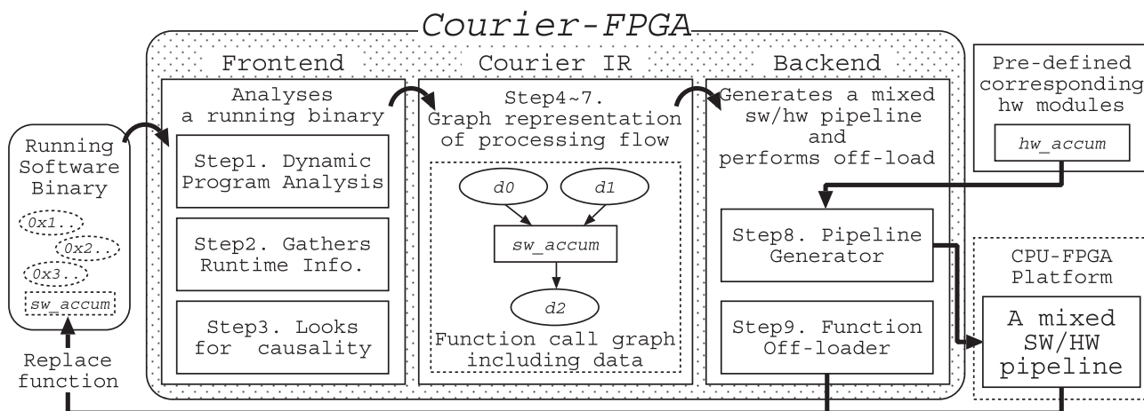
Fig. 1 Overview and work-flow of Courier-FPGA: the Frontend analyzes the running binary (Step1, 2 and 3) and then generates a function call graph including input-output data and a Courier Intermediate Representation (IR) . The user refers to the graph and results, decides which parts to off-load and rewrites IR if needed (Steps 4, 5, 6 and 7). After that, the Pipeline Generator builds a mixed sw/hw pipeline (Step 8). Finally, the Function Off-loader replaces function and off-loads it to the accelerator (Step 9).
