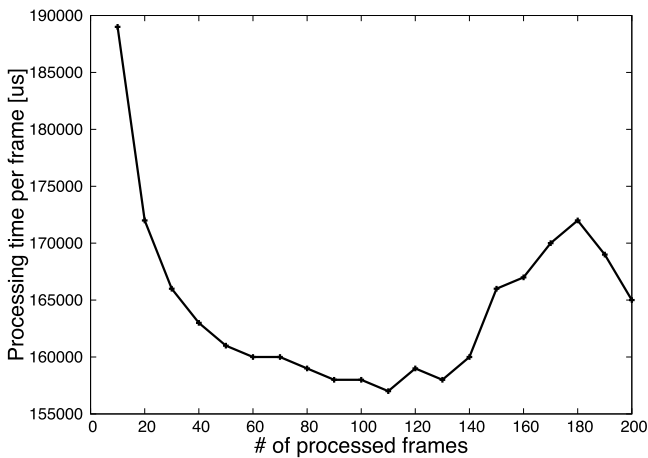
Fig. 5 Processing time per frame fluctuates a little since Intel TBB's pipeline is based on a thread pool. It works differently from a pure hardware pipeline.
