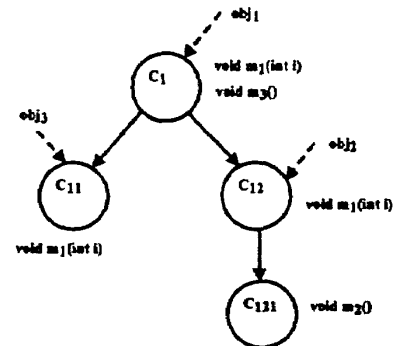
Figure 1: Class Taxonomy
