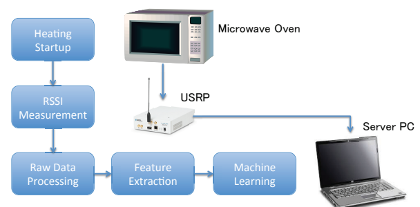
Fig. 3 The workflow block diagram of the proposed recognition system.
