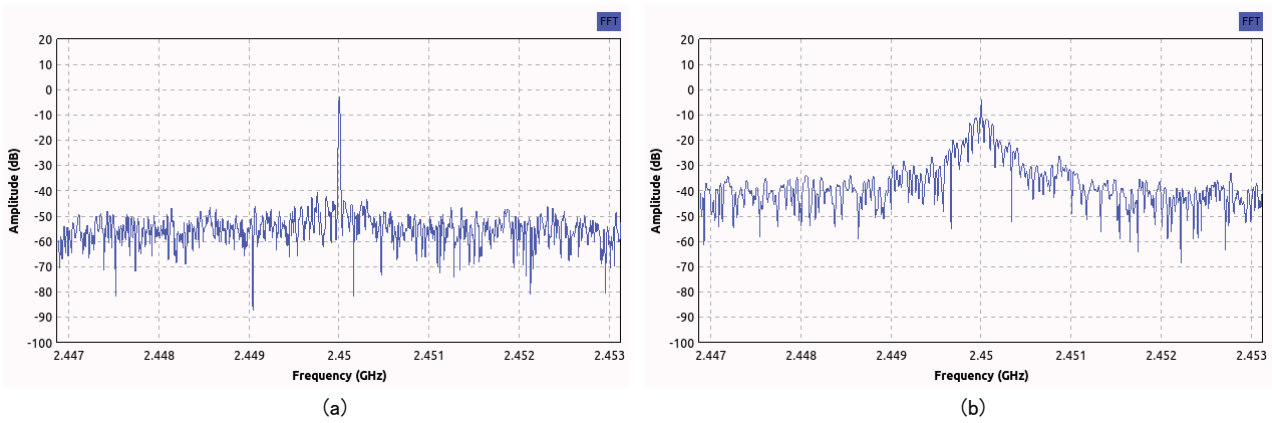
Fig. 11 Spectrum of two microwave ovens. (a) National NE-EZ2. (b) Panasonic NE-EH225.
