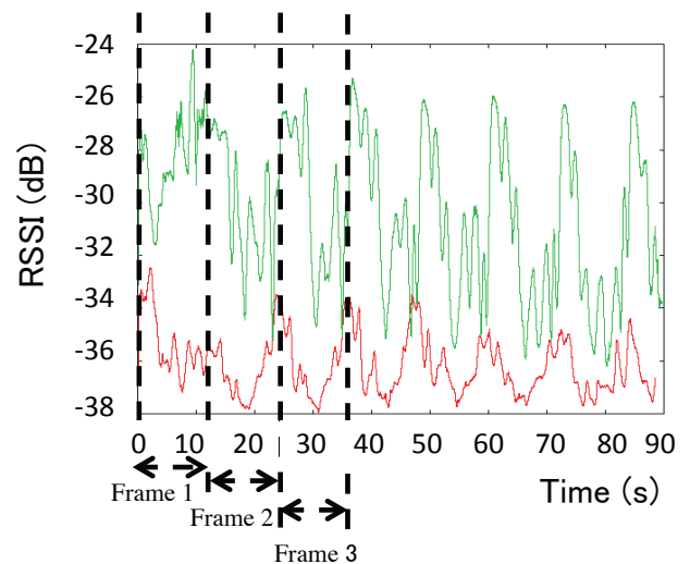
Fig. 9 First three frames of raw data with the recognition distance of 0.3 m and the down sampling frequency of 2 kHz. Red: pizza. Green: French fries.
