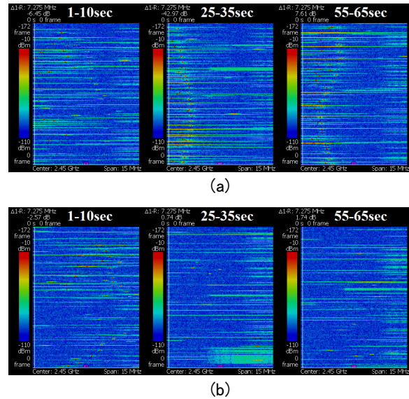
Fig. 7 Spectrogram of the microwave oven leakage when heating (a) water and (b) French fries.
