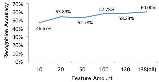
Fig. 12 The relationship between top feature amount and recognition accuracy for the case of 138 features with 5-m recognition distance and 2-kHz down sampling frequency.
