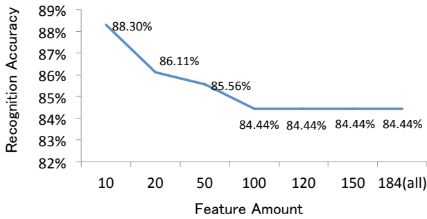
Fig. 10 The relationship between top feature amount and recognition accuracy for the case of 184 features with 5 m recognition distance and 2 kHz down sampling frequency.
