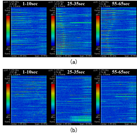
Fig. 7 Spectrogram of the microwave oven leakage when heating (a) water and (b) French fries.
