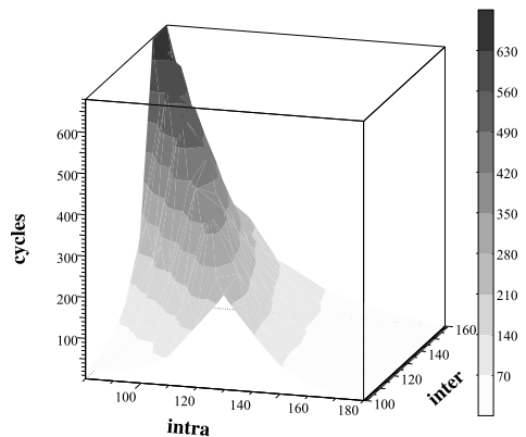
Fig. 7 Median cycles (5 agents with 20 nodes each, random 3col, with multi-ABT).
