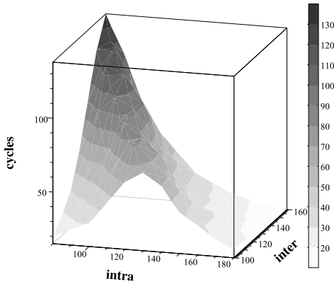
Fig. 9 Median cycles (5 agents with 20 nodes each, solvable 3col, with multi-ABT).
