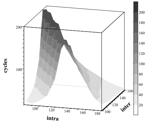
Fig. 5 Median cycles (2 agents with 50 nodes each, random 3col, with multi-ABT).
