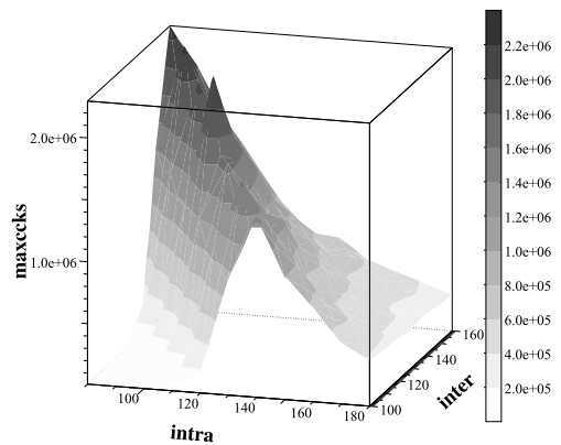
Fig. 6 Median maxccks (2 agents with 50 nodes each, random 3col, with multi-ABT).
