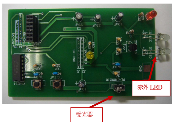
図2 試作赤外線リモコン送受信器ボード Figure 2 Test Fabricated IR-Transceiver Board.
