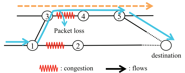
Fig. 2 Load balancing using IP Fast Reroute [16].
