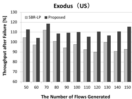
Fig. 13 Throughput in Exodus network.
