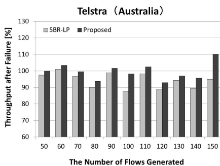
Fig. 10 Throughput in Telstra network.
