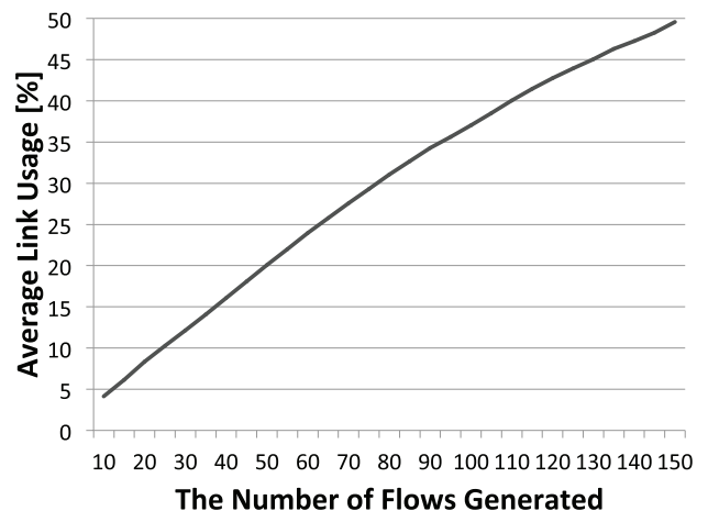
Fig. 6 Average link occupancy in normal state.
