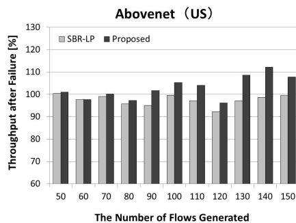
Fig. 14 Throughput in Abovenet network.
