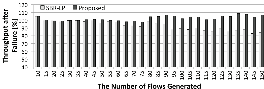
Fig. 5 Throughput with various random network load (average of 30 trials).
