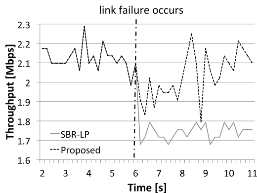
Fig. 8 Throughput in time series.
