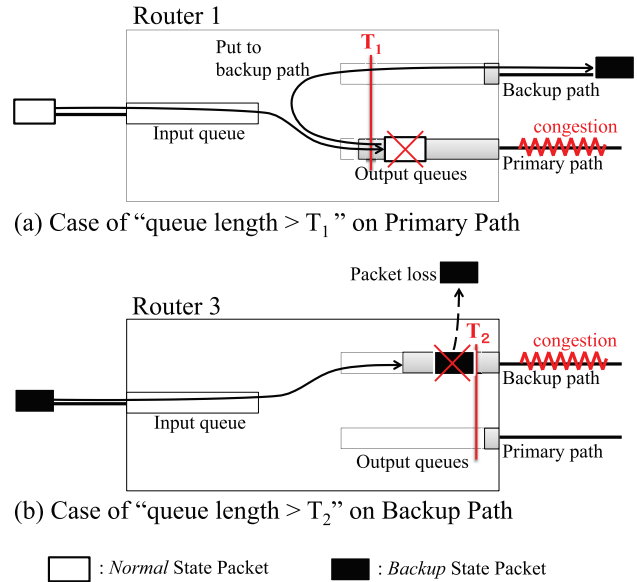
Fig. 3 Load balancing behavior based on queue length.
