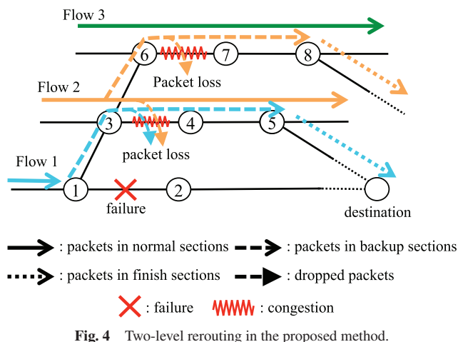
Fig. 4 Two-level rerouting in the proposed method.
