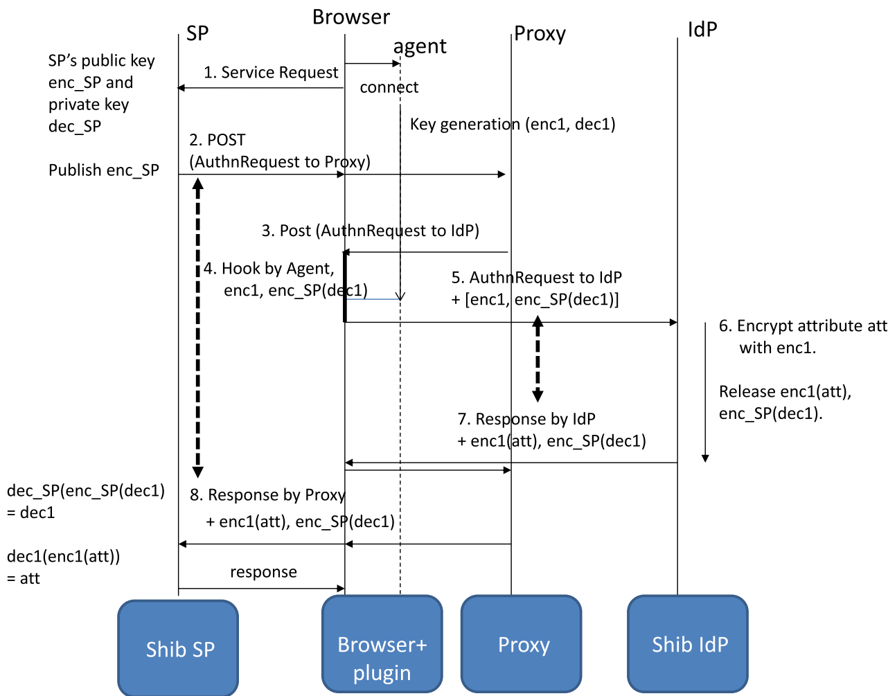
Fig. 2 WebSSO profile of using Ephemeral Key Pairs.
