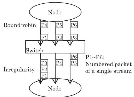
Fig. 3 Outline of round-robin distribution.
