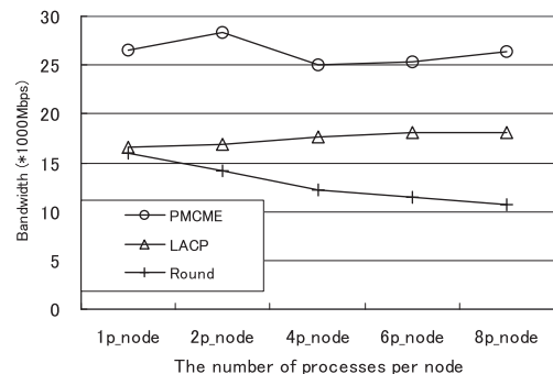
Fig. 13 Many-to-many bandwidth.
