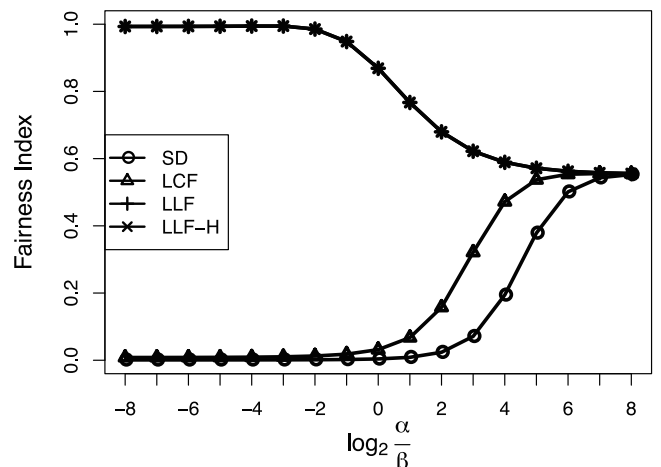
Fig. 11 Load distribution by \log_2 \frac{\alpha}{\beta} .
