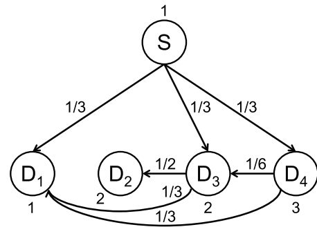
Fig. 7 An example of the LCF method.
