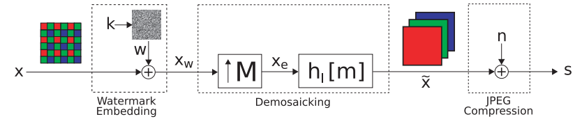
Fig. 4 Watermarking embedding and image processing pipeline.
