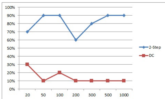
Fig. 10 The success rate in different size networks.
