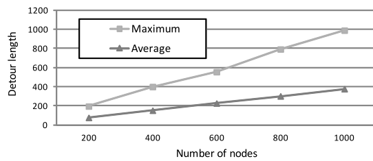
Fig. 16 Detour path length on serial graph.
