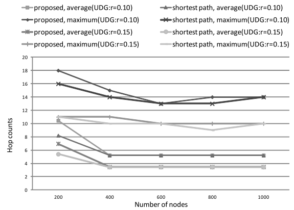
Fig. 13 Average hop counts and maximum hop counts.
