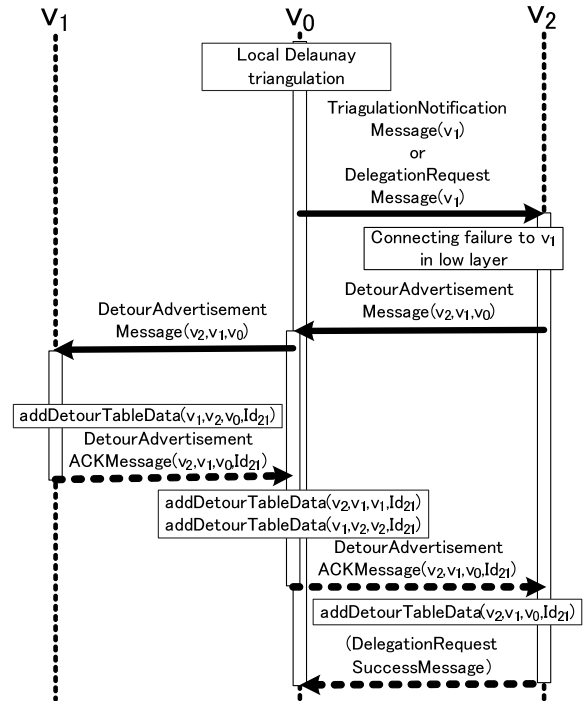
Fig. 10 Detour table construction sequence diagram.
